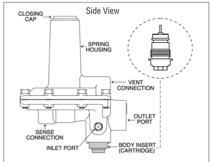
Figure 1 - The Series 20L Flowgrid™ Pilot.
