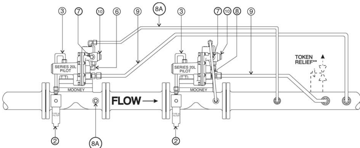
Figure 13 - Standby Monitor with Differential Pressure Less than 60 psig
