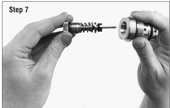
Figure 30 - Insert the assembly into the Body Insert- the orifice should "snap" into place.
