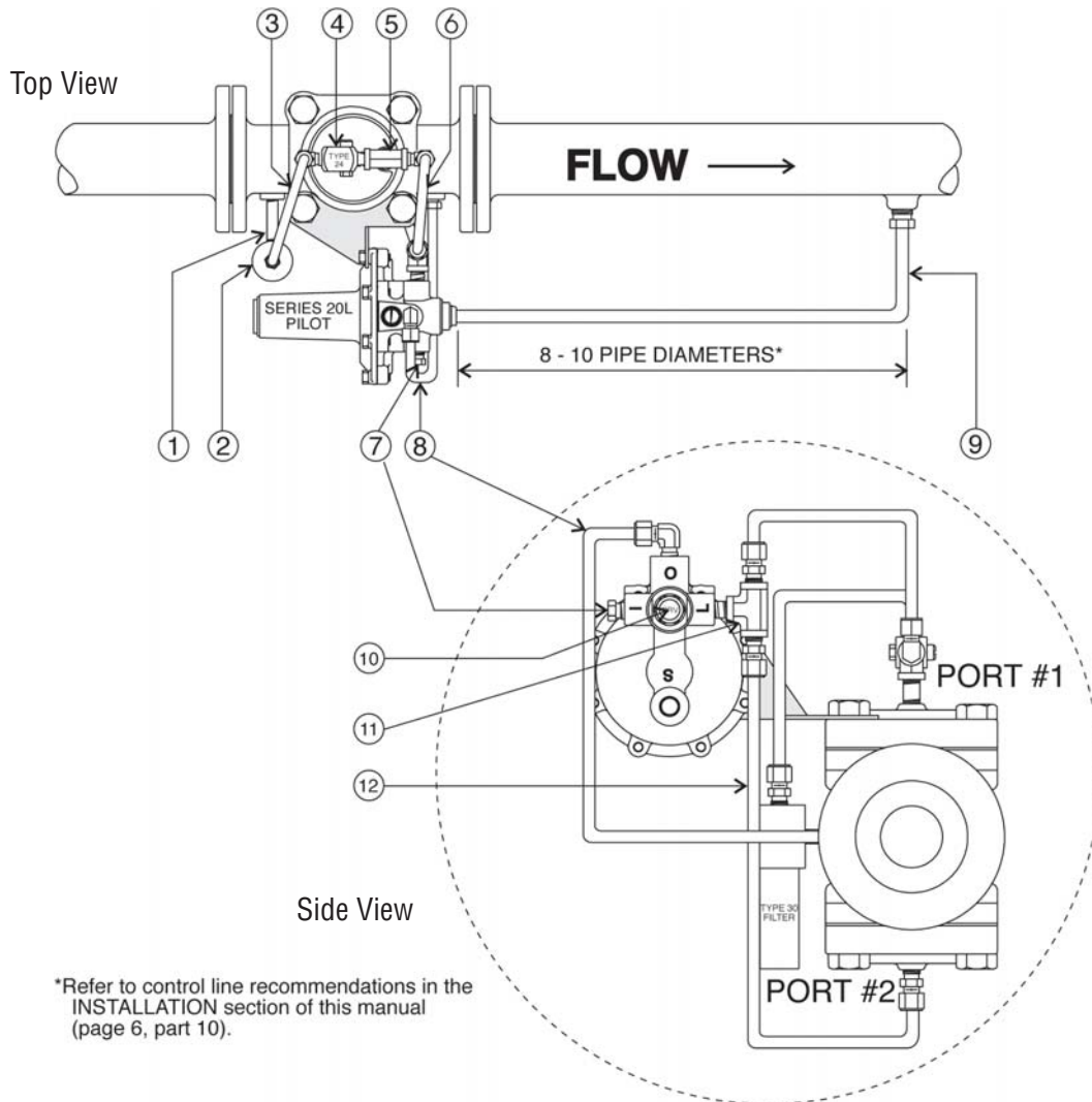
Figure 10 - Dual Port / Single Pilot (Pressure Reducing Valve)
