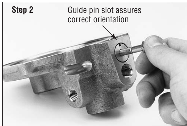
Figure 23 - Use a 5/16"-18 UNC bolt to push the Pivot plug / Lever assembly into place. Remove the bolt when complete.
