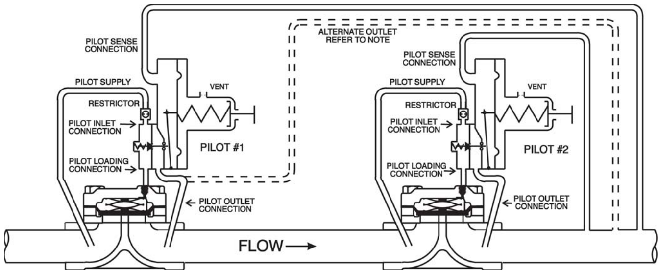
Figure 15 - Standby Monitor Schematic.
