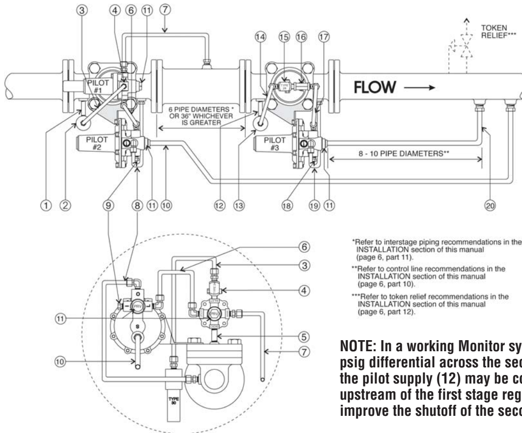
Figure 14 - Working Monitor (Also Refer to Schematic on Page 14)
