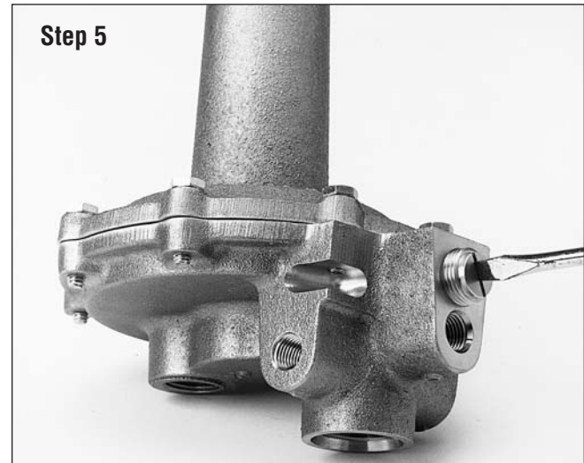
Figure 20. Remove the Threaded Retainer Plug.
