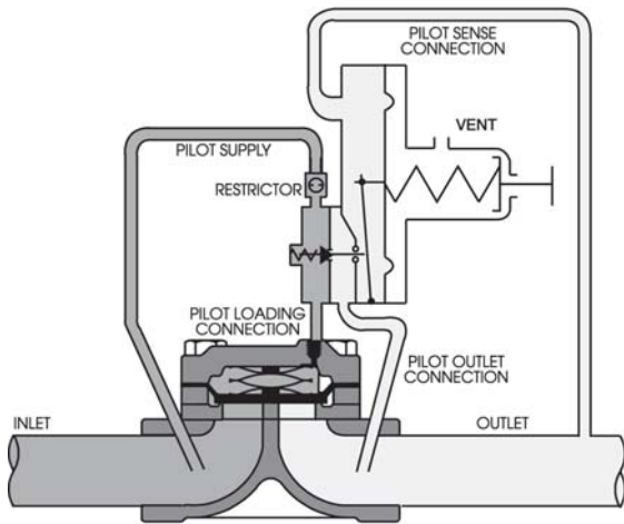
Figure 6 - Pressure Reducing Configuration Fully Closed.
