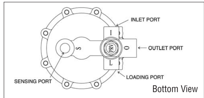
Figure 2 - The Series 20L Flowgrid™ Pilot.
