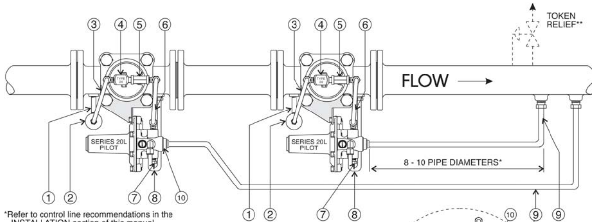
Figure 12 - Standby Monitor with Differential Pressure Greater than 60 psig
