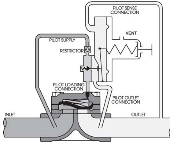
Figure 7 - Pressure Reducing Configuration Partially Open.
